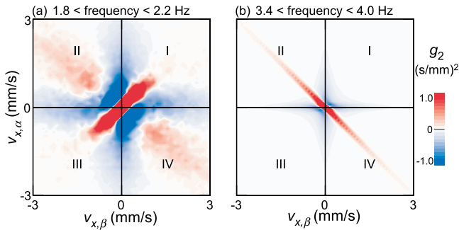
FIG. 4 (color online). Two-particle correlation function g_2 recalculated using frequency-filtered velocity time-series data. Different frequency bandpasses were chosen for (a) and (b) to correspond to the two peaks in the spectrum of Fig. 3(b). Features in g_2 are distinctly different for (a) and (b), which indicates that g_2 is dominated by the collective effects of two kinds of oscillations. To help distinguish the type of oscillations, the four quadrants I–IV are labeled as in Fig. 3(a). Comparing (a) and (b) to the labels in Fig. 3(a), we find that correlations arising from oscillatory motion at \approx 2.0 Hz in (a) correspond to the center-of-mass motion, while correlations at \approx 3.7 Hz in (b) correspond to the breathing mode. As in Fig. 2(c), positive and negative correlations are shown in red and blue (top and bottom of the color scale), respectively.
