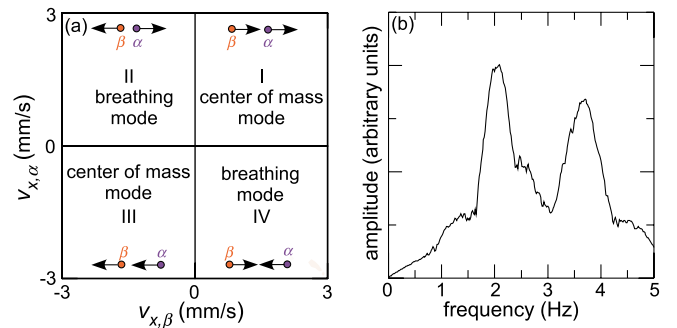
FIG. 3 (color online). (a) Labeling scheme for the quadrants of phase space according to the two types of oscillatory motion. (b) The frequency spectrum for the particle velocities, which is calculated as the square of the fast Fourier transform of the velocity time series for a particle. The frequency spectrum has two peaks, at 2.0 and 3.7 Hz, which we will identify as the center-of-mass and breathing modes, respectively.
