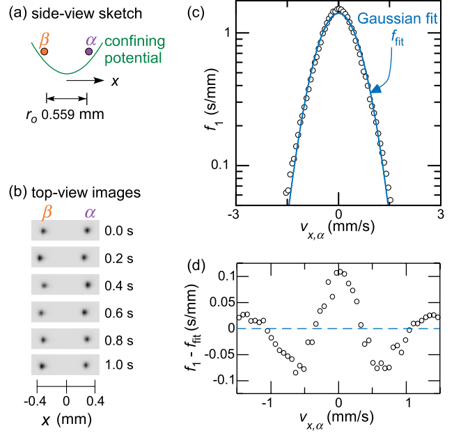
FIG. 1 (color online). (a) A side-view sketch of two microparticles, labeled \alpha and \beta , in a harmonic confining potential. The microparticles move mainly along the x axis, and they oscillate in the confining potential. (b) Sequence of top-view images of the two microparticles [24] recorded by video microscopy, showing their small displacements with time. (c) The one-particle velocity distribution f_1(\alpha) for microparticle \alpha is presented as a histogram of velocity observations. It is slightly non-Gaussian; the deviation from a Gaussian fit is shown in (d) with an expanded scale.
