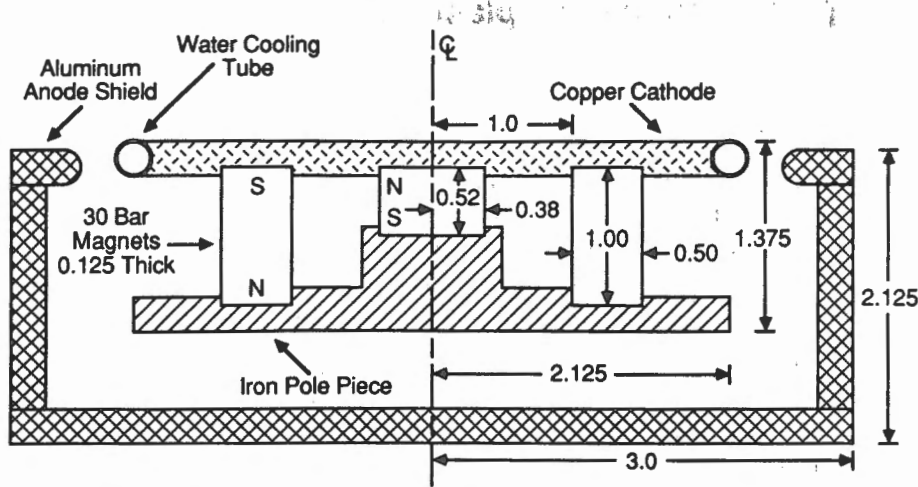
FIG. 1. Schematic drawing of the magnetron. All dimensions are in inches.
