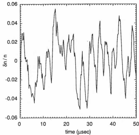
FIG. 3. Time history of density fluctuations taken at position 1 for a discharge current of 0.127 mA. Points were taken every 0.2 \mu\text{s} , and the first 251 points out of 8192 recorded are shown.
