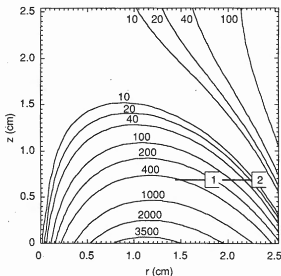
FIG. 2. Contour plot of the calculated effective magnetic potential \psi = q^2 A_\theta^2 / (2m) , seen by an electron with P_\theta = 0 . Contour values are in volts. The presence of the plasma sheath prevents electrons from escaping to the cathode. Probe positions 1 and 2 are indicated. The surface of the cathode is at z = 0 cm.
