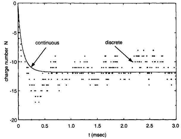
Fig. 3. Temporal evolution of charge number N = Q/e for, aT_e = 10 nm eV, T_i/T_e = 0.05 , m_i = 1 amu and n = 10^{15} \text{ m}^{-3} . Note that the discrete charging model reveals fluctuations about the smooth curve predicted by the continuous model.
