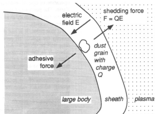
Fig. 1 Sketch of forces acting on a dust particulate attached to a large body (not to scale).
