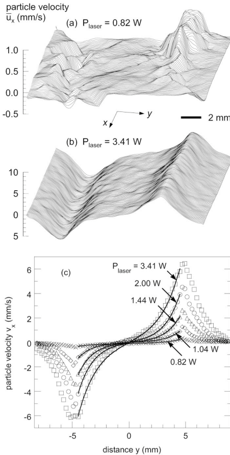
FIG. 2. Particle velocity data. Map (a), averaged over 64 frames at the onset of plastic flow, shows particle movement localized near the laser footprints. Map (b), averaged over 256 frames at the highest laser power, shows a fully developed shear flow that has no variation with x . Experimental profiles (data points) (c) are with fits to the Navier-Stokes model (curves), as used to calculate the kinematic viscosity of the particle suspension.
