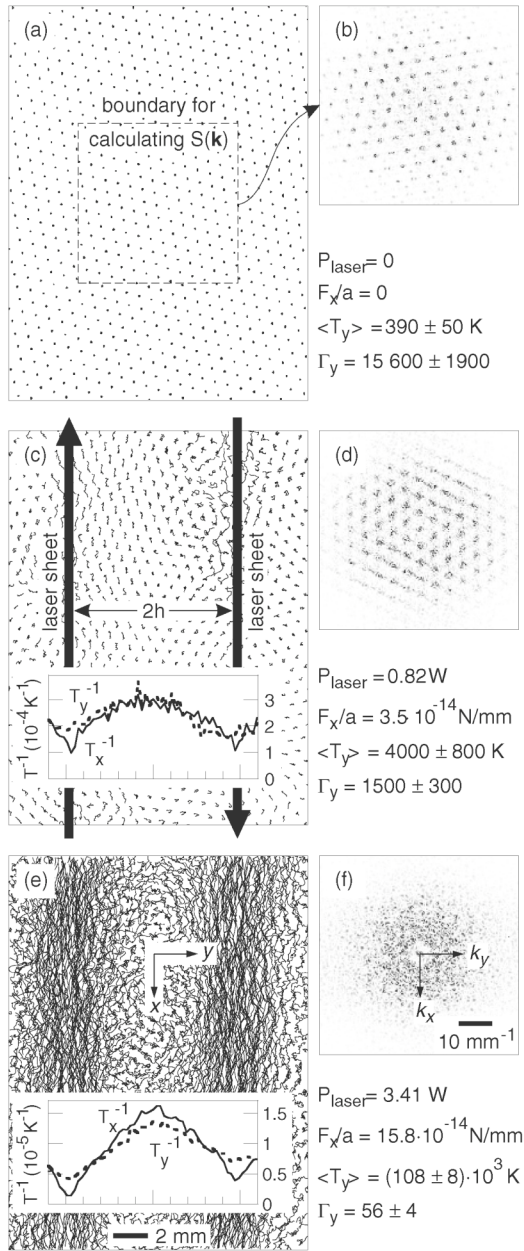
FIG. 1. Particle suspension at three levels of shear stress applied by a pair of counterpropagating laser sheets in a planar Couette configuration. Panels (a), (c), and (e) are top views with shear stress that is zero, moderate, and high, respectively. The snapshot of the undisturbed suspension (a) shows a highly ordered triangular lattice. At the onset of plastic flow (c), particle trajectories reveal localized hopping. In a fully developed shear flow (e), the trajectories show particles moving significantly everywhere. Profiles of the inverse particle temperature T_x^{-1} and T_y^{-1} are shown in the insets. The static structure factor S(\mathbf{k}) was computed as the Fourier transform of the raw bitmap images as in (a). The peaks in S(\mathbf{k}) are distinctive for an undisturbed lattice (b); they are broadened and then diffuse at progressively higher levels of shear (d),(f). The particle suspension's parameters here and in Fig. 2 correspond to Experiment 1 in Table I. We calculated \eta , \langle T_y \rangle , and \Gamma_y using data in the range -h < y < h .
