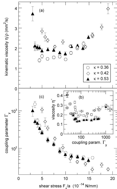
FIG. 3. Results for kinematic viscosity \eta / \rho , as functions of the shear stress (a) and coupling parameter \Gamma_y (b). The latter two parameters were not varied independently, but were related as shown in (c). There is a broad minimum in viscosity in the range 70 < \Gamma_y < 700 . In (b), to allow comparison to theory, we normalized the viscosity as \eta^* = \eta / (\rho \omega_{pd} a^2) , where \omega_{pd} \equiv [Q^2 / 2\pi \epsilon_0 m a^3]^{1/2} for two dimensions [11].
