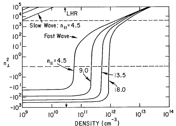
FIG. 1. Dispersion relation of the fast and slow waves. The unbounded cold-plasma dispersion-relation solutions are shown for B_0 = 4.47 kG, f = 18 MHz, and m_i = 4 amu. This plot is made of two log-log plots joined together: one for positive, i.e., propagating, values of k_{\perp}^2 , and one for negative values. The upper horizontal dashed line gives an estimate of the density required to fit a half wavelength across the diameter of the ACT-I vessel. (The density actually required is less because rounded density profiles allow certain eigenmodes to propagate with less density.) The lower-hybrid resonance density is indicated by arrows.
