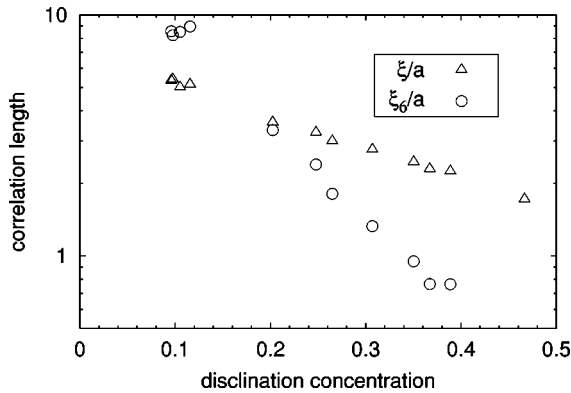
FIG. 11. Correlation lengths \xi/a and \xi_6/a versus disclination concentration.
