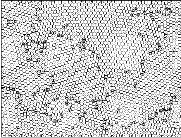
(c) disclination concentration = 0.26
