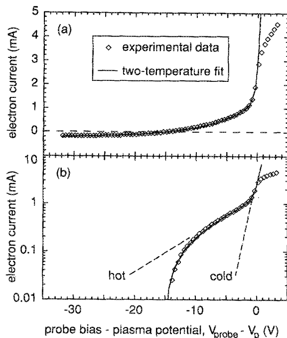
FIG. 2. Measured two-temperature probe characteristic taken at r = 1.2 cm, z = 2.5 cm. In (a) the electron current is plotted on a linear scale, and in (b) on a logarithmic scale. The two slopes shown by the dashed lines in (b) are due to the presence of hot and cold electron components. The solid line gives the fit to a two-temperature model for T_e^{\text{cold}} = 0.47 eV, n_e^{\text{cold}} = 2.4 \times 10^{16} \text{ m}^{-3} , T_e^{\text{hot}} = 6.8 eV, and n_e^{\text{hot}} = 0.68 \times 10^{16} \text{ m}^{-3} .
