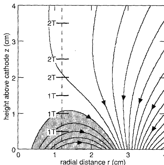
FIG. 1. Computed magnetic field lines for the magnetron, with the magnetic trap shaded. The positions at which probe measurements were made are shown by the horizontal lines at r = 1.2 cm. The length of these lines gives the length of the probe tip. At each of these points we have indicated whether one or two electron components were observed, using "1T" or "2T," respectively. Note that there are both hot and cold electrons outside the magnetic trap, while there are only hot electrons in the trap.
