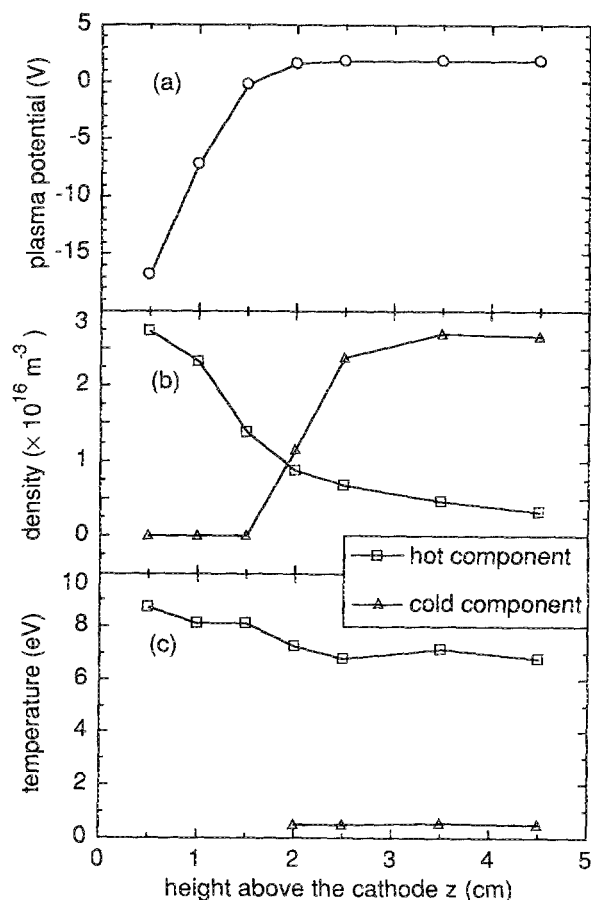
FIG. 3. (a) Plasma potential, (b) electron density, and (c) electron temperature plotted against the height above the cathode, z . There is a steep potential gradient (i.e., large electric field) in the magnetic trap. The hot electron density is largest in the magnetic trap and decreases as z is increased. In contrast, the cold electron density is large outside the trap and negligible inside. The average hot electron temperature is 7.6 eV, while the average cold electron temperature is 0.50 eV.
